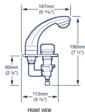
SINGLE FAUCET COLD ONLY
