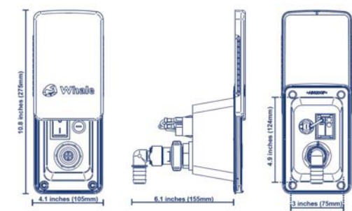
4 IN 1 FITTING
