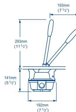
BP0535 THRU DECK
