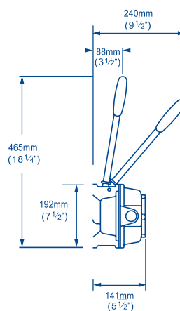
BP0527 BULKHEAD
