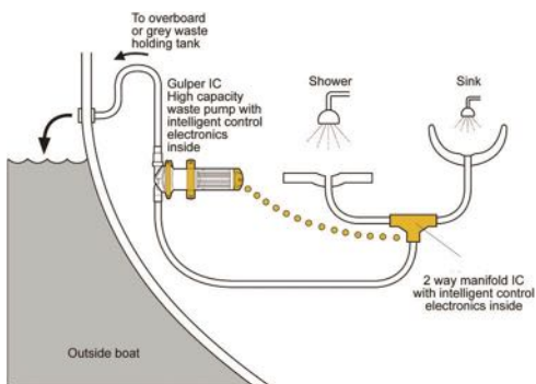
TYPICAL INSTALLATION
