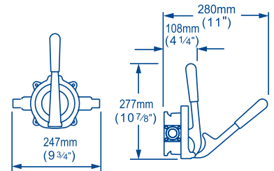
On Deck/Fixed Handle BP9005
