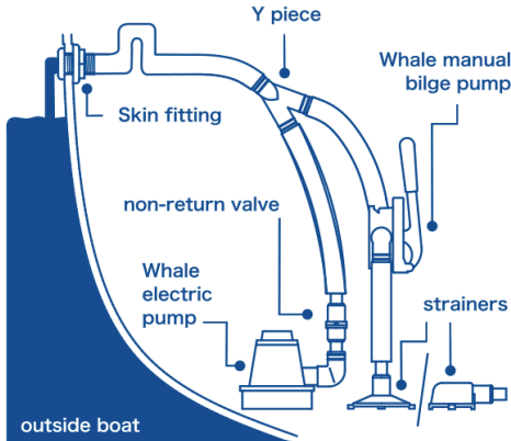
TYPICAL INSTALLATION
