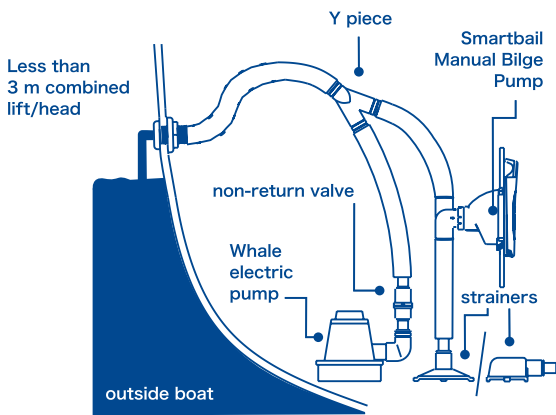
TYPICAL INSTALLATION
