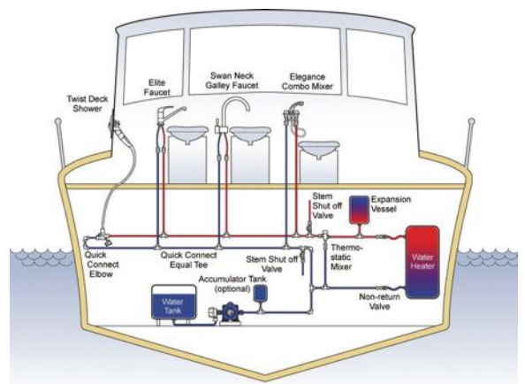
TYPICAL INSTALLATION
