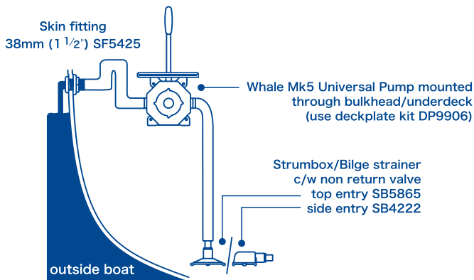
TYPICAL INSTALLATION
